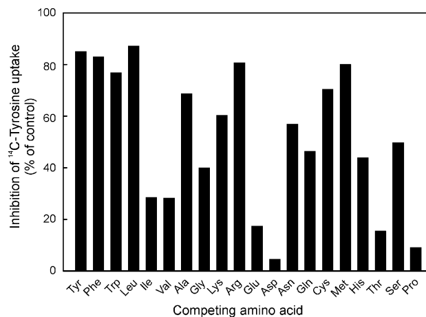
Fig. 4. Competition of unlabeled amino acids for uptake of [ ^{14} C]tyrosine by S. cerevisiae strain M4054 expressing ArlP. [ ^{14} C]tyrosine was present at a final concentration of 25 \mu M, and the indicated unlabeled amino acids were added in a 10-fold excess. The rate of uptake was determined after 3 min and results shown are the means of three independent experiments.
